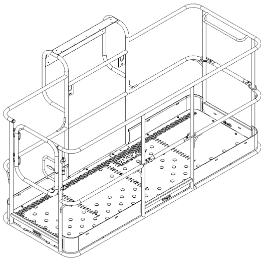
(1) Side Swing Gate Platform
